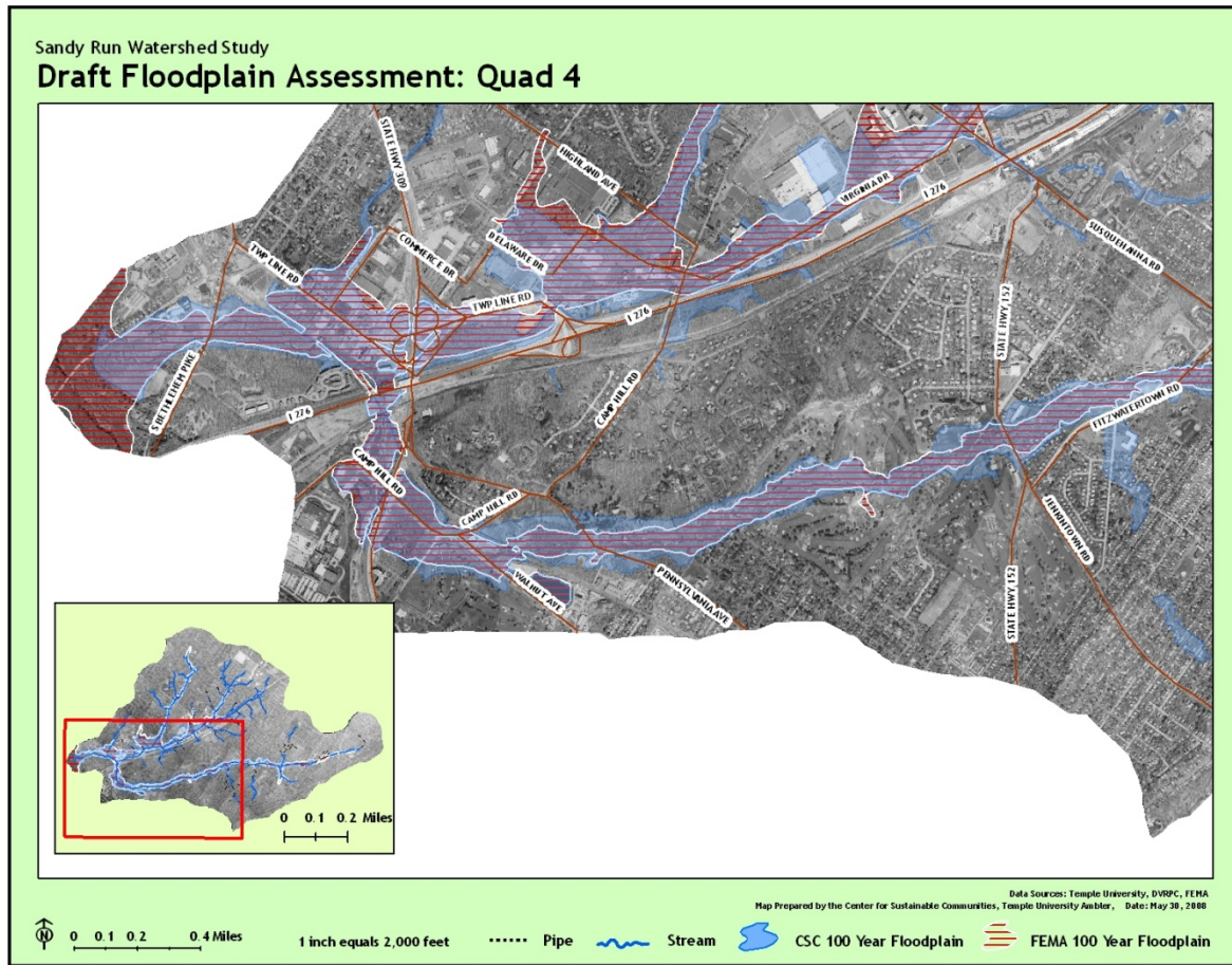
Figure 4 - 100-Year Floodway Comparison, Quad 4
